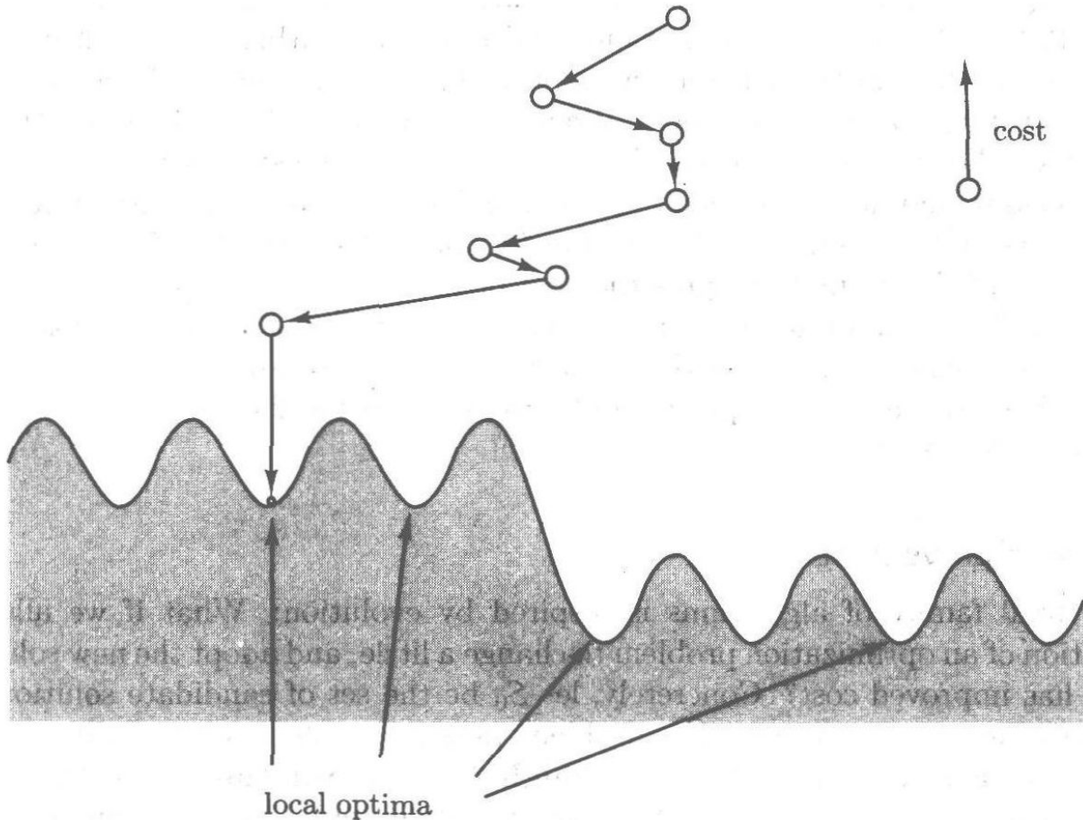
Figure 7-16: Once the neighborhood relation has been fixed, the solutions of an optimization problem can be pictured as an energy landscape , in which local optima are depicted as valleys. Local improvement heuristics jump from solution to solution, until a local optimum is found.
