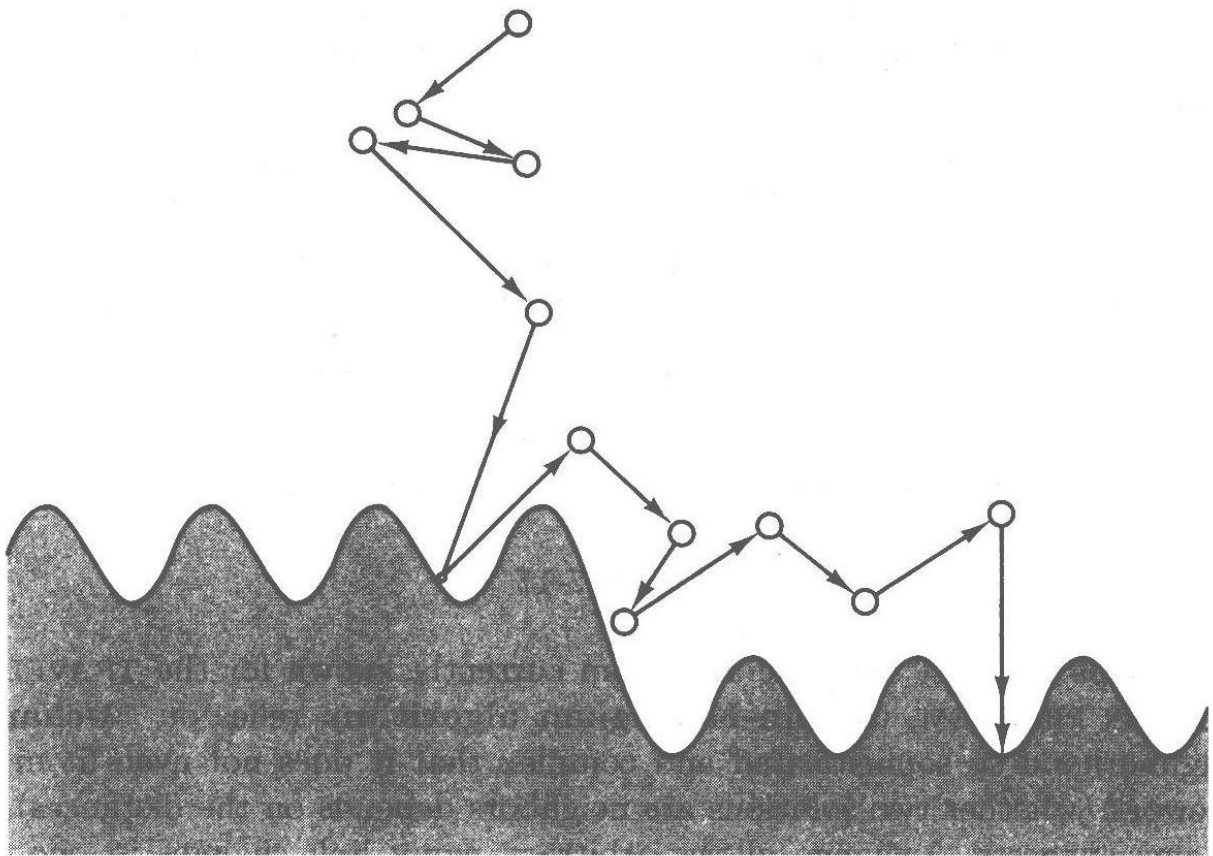
Figure 7-18: Simulated annealing has an advantage over the basic local improvement algorithm because its occasional cost-increasing moves help it avoid early convergence in a bad local optimum. This often comes at a great loss of efficiency.
