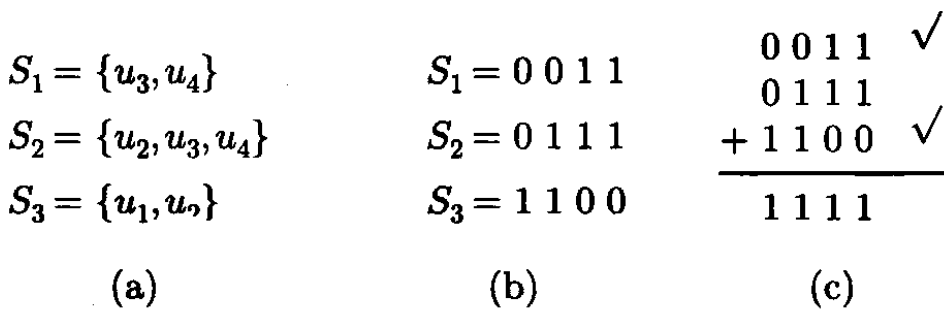
Figure 7-8: From sets (a) to bit vectors (b) to integer addition in base m (c)
